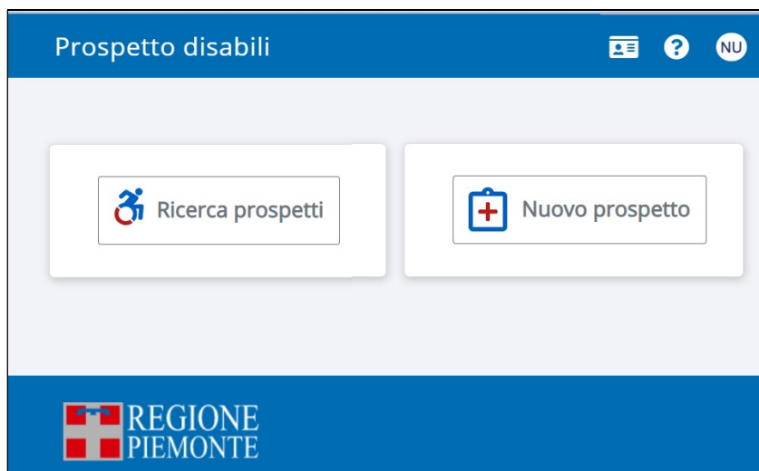
Figura 7 - Homepage
