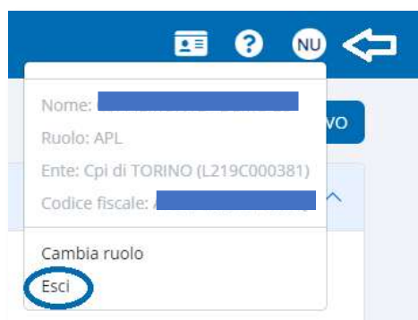
Figura 35 – Logout
